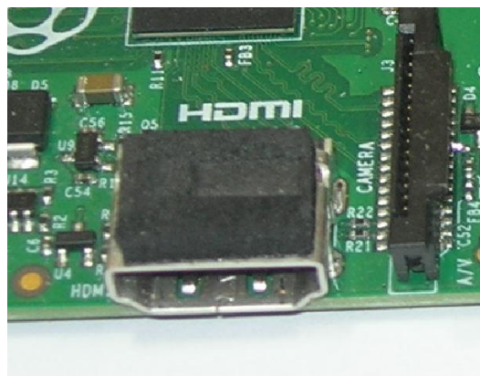
Figure 3 Black Rubber Spacer glued on the HDMI connector
