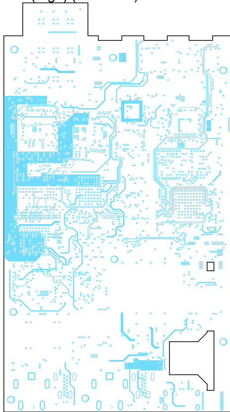
Int3 (Sign) (Scale 1:1)
