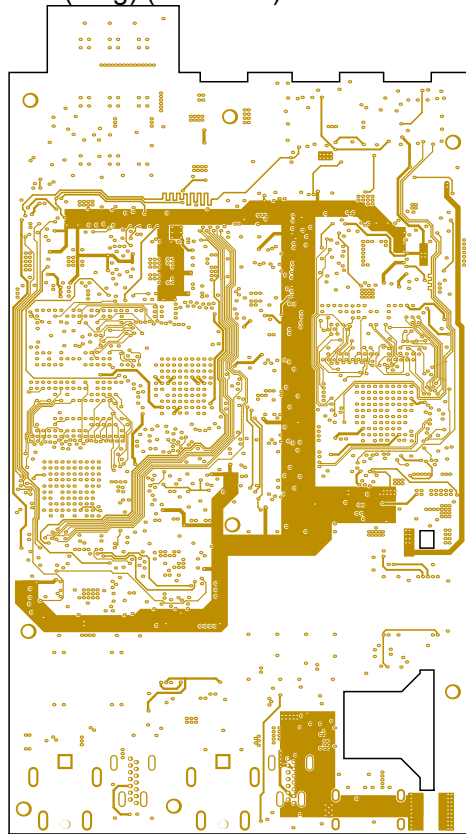
Int2 (Sing) (Scale 1:1)
