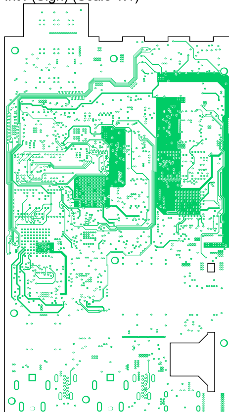
Int4 (Sign) (Scale 1:1)
