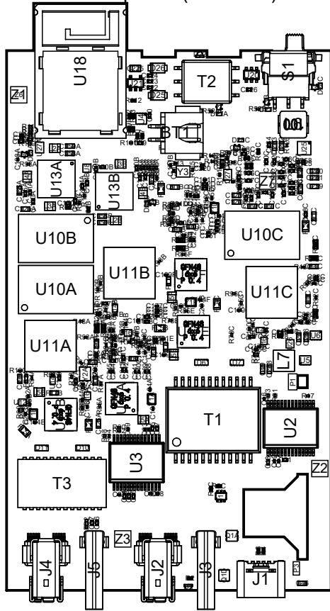
View from Top side (Scale 1:1)
