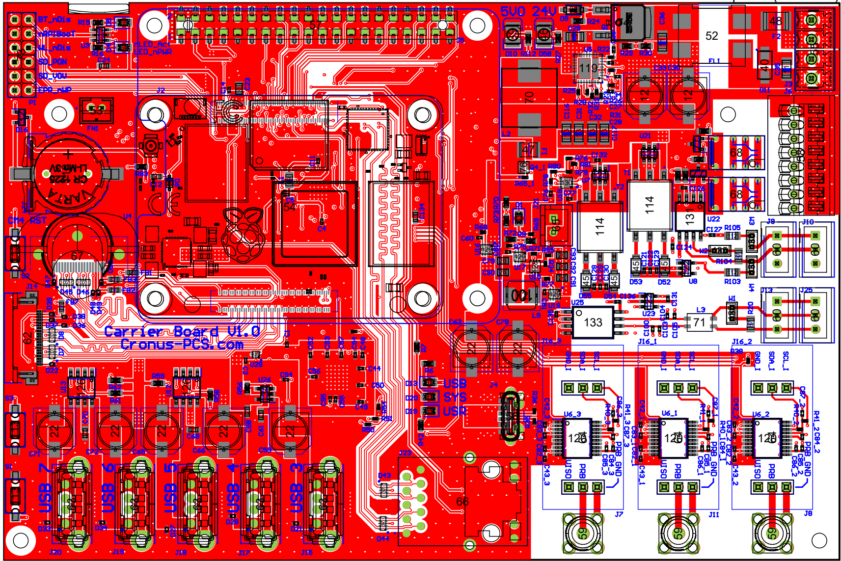
View from Top side (Scale 3:2)
