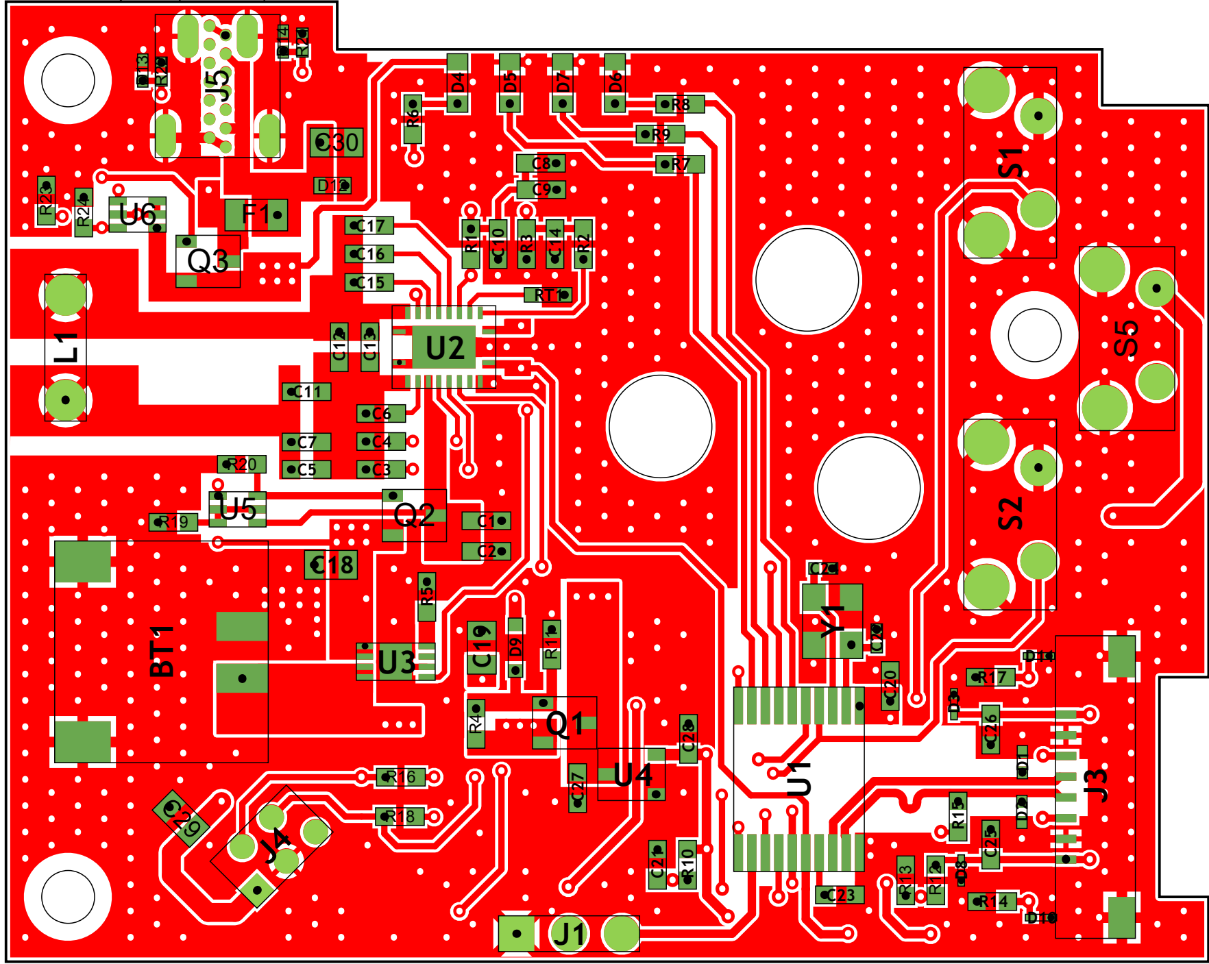
View from Top side (Scale 4:1)
