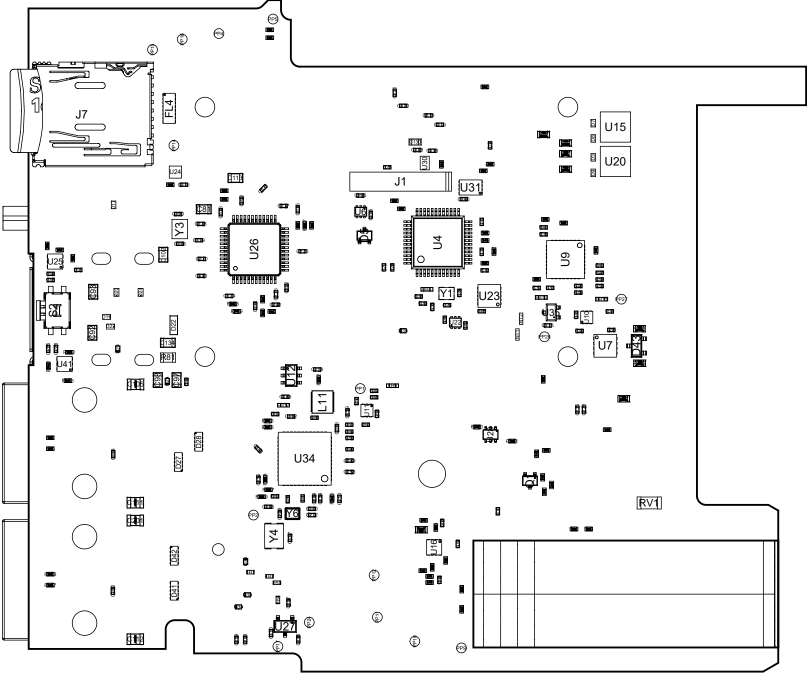
View from Bottom side (Scale 2:1)
