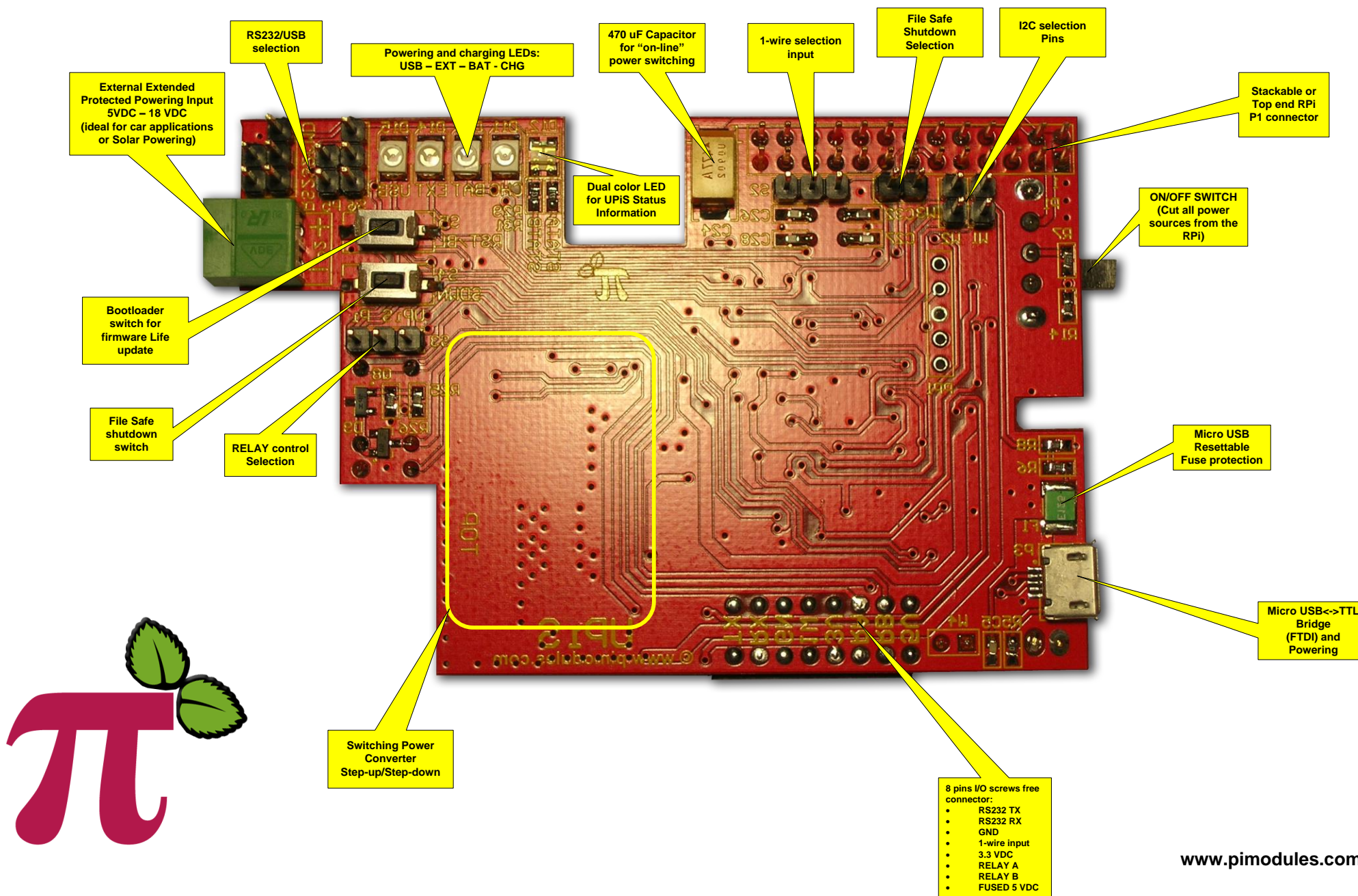
TOP PCB View
