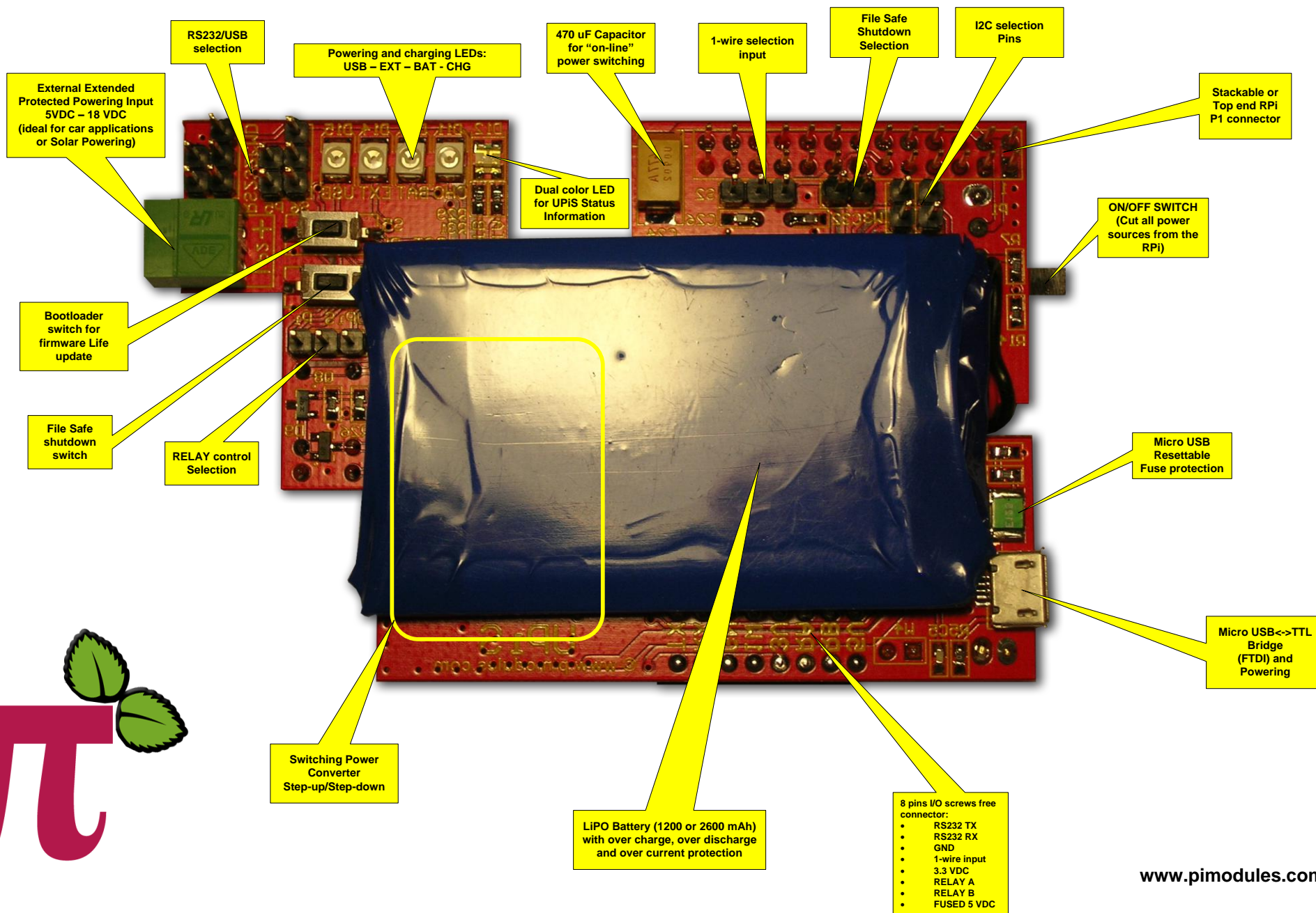
TOP PCB with battery View
